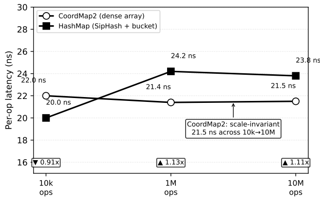
Figure 6: Get latency across three scales: CoordMap2 (flat) vs HashMap (rising with memory pressure)
