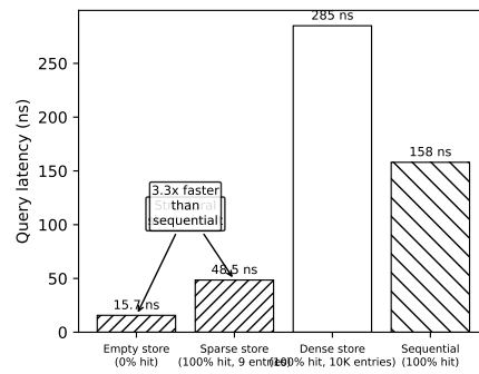
Figure 9: CoordCube vs sequential lookup: hit-rate crossover
