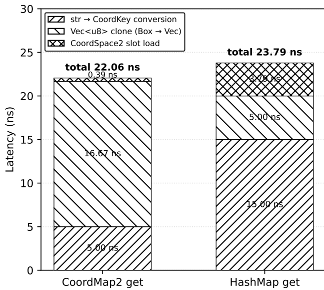
Figure 3: Latency breakdown: CoordMap2 get vs HashMap get. CoordMap2 pays str-to-CoordKey conversion once at the API boundary; the slot load itself is 0.39 ns. HashMap pays SipHash on every access with no structural benefit.
