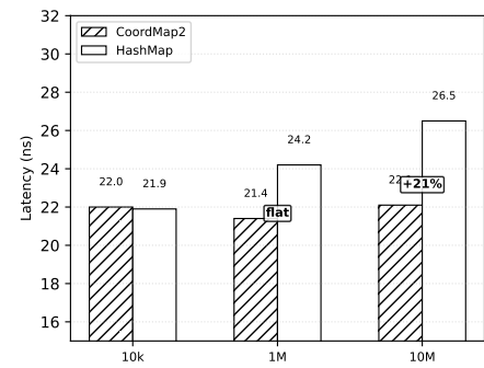
Figure 10: Scale-invariant KV get latency: CoordMap2 vs HashMap
