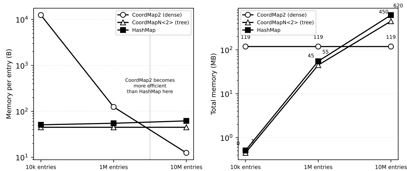
Figure 1: Memory efficiency across three scales: CoordMap2 fixed-cost amortization vs proportional scaling of CoordMapN and HashMap.
