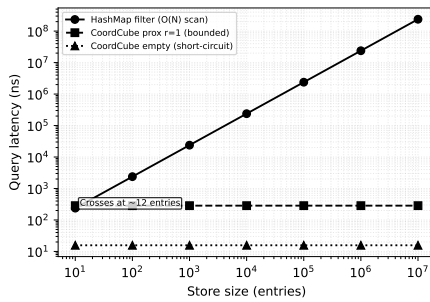
Figure 8: Query cost vs store size: Coord- Cube proximity vs HashMap filter
