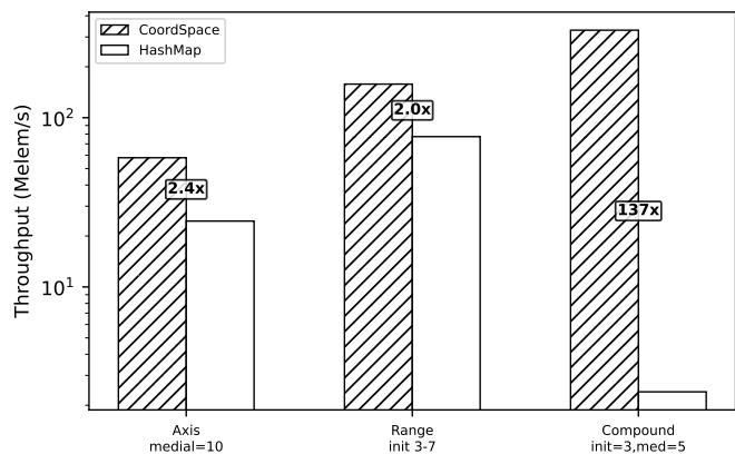
Figure 12: Spatial query throughput
