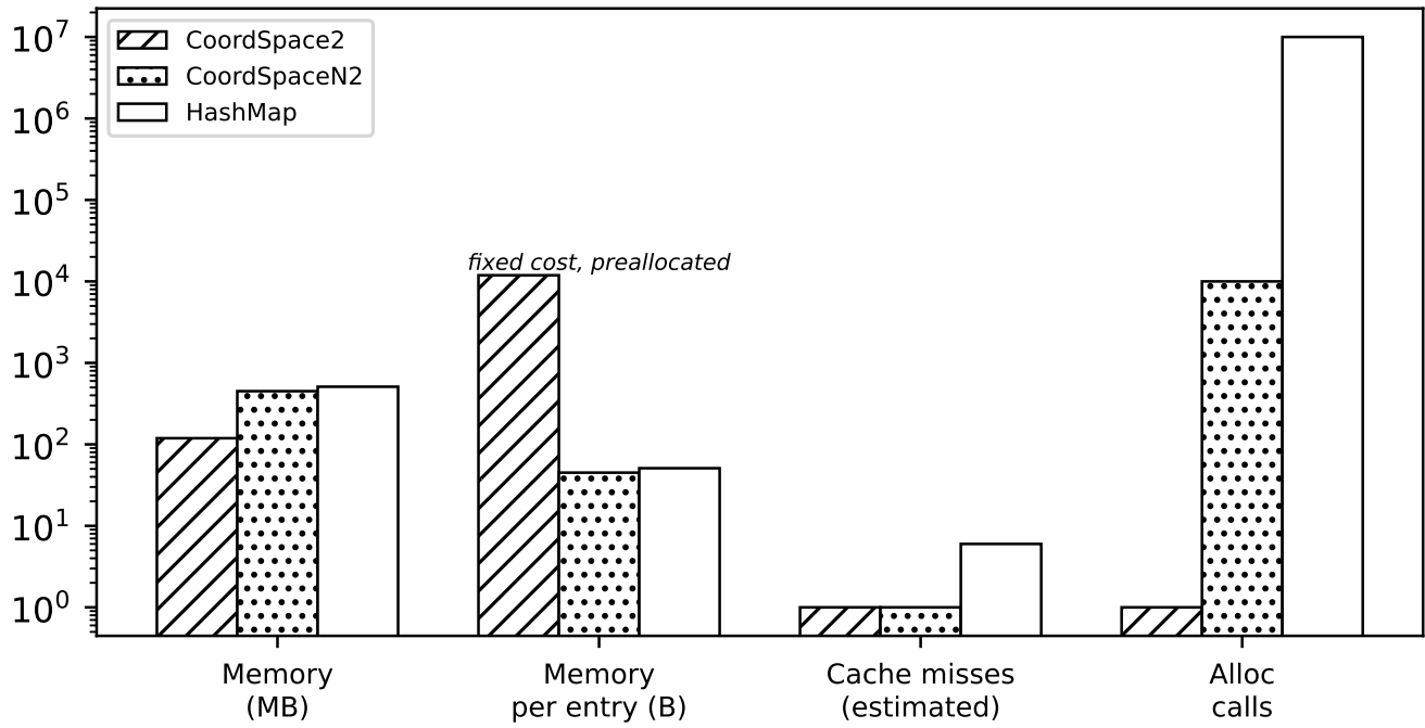
Figure 2: Resource usage at 10K entries: CoordSpace2 (dense), CoordSpaceN2 (tree), and HashMap. Dense coordinate space uses a fixed 119 MB regardless of occupancy, making per-entry cost (11900 B) high at low density but allocation-free. Tree scales per-prefix: 45 B/entry with minimal allocations. HashMap pays per-entry malloc overhead (51 B/entry) and accumulates 10M allocation calls.
