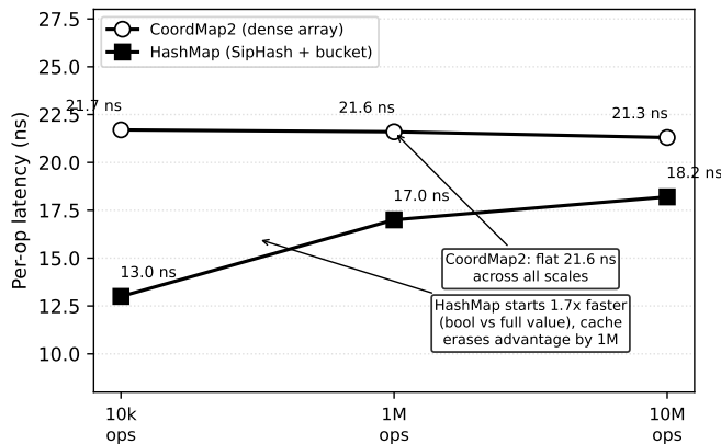
Figure 7: Contains key latency across three scales: CoordMap2 (flat) vs HashMap (bool advantage narrows under cache pressure)
