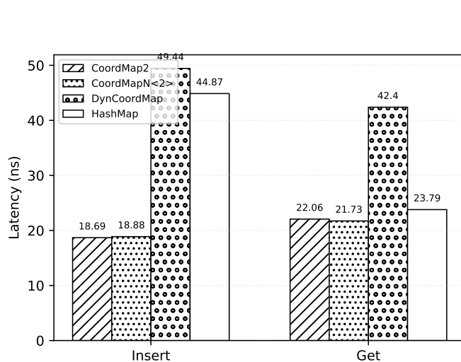
Figure 5: Single insert and get latency — all four variants
