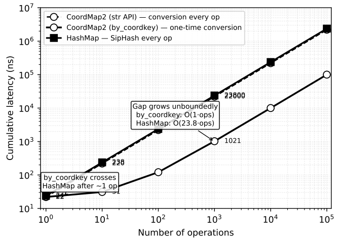
Figure 4: Cumulative cost model: CoordMap2 with by_coordkey API pays the conversion cost once and then accesses at slot-load cost. HashMap pays SipHash on every operation.
