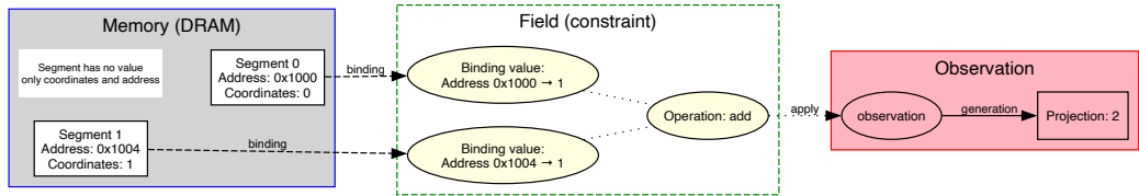
Figure 5: 1+1=2 under SSCCS
